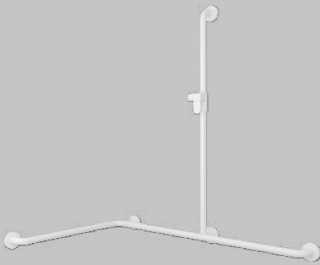
VICARE FUNCTION DUSCHGRAB RAIL WITH SHOWER HOLDER IN T-FORM, MADE OF POWDER-COATED ALUMINIUM, WITH VERTICAL AND HORIZONTAL HANDLE, SHOWER CAN BE ADJUSTED IN HEIGHT WITH ONE HAND
