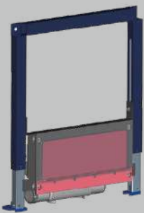
VICONNECT INSTALLATION SYSTEMS WALL OUTLET UNIT INCL. FRAME FOR DRY-WALL CONSTRUCTION, 525 x 510 x 135 mm
